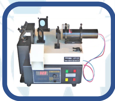
Thermal Expansion Experiment
